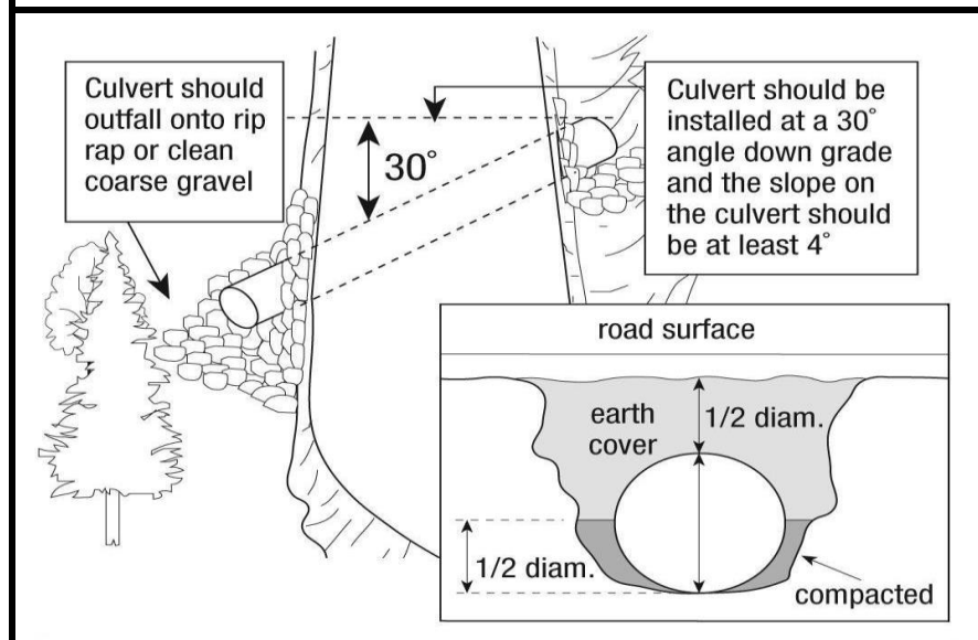
Figure 12-8 Installation of a cross-drainage culvert
